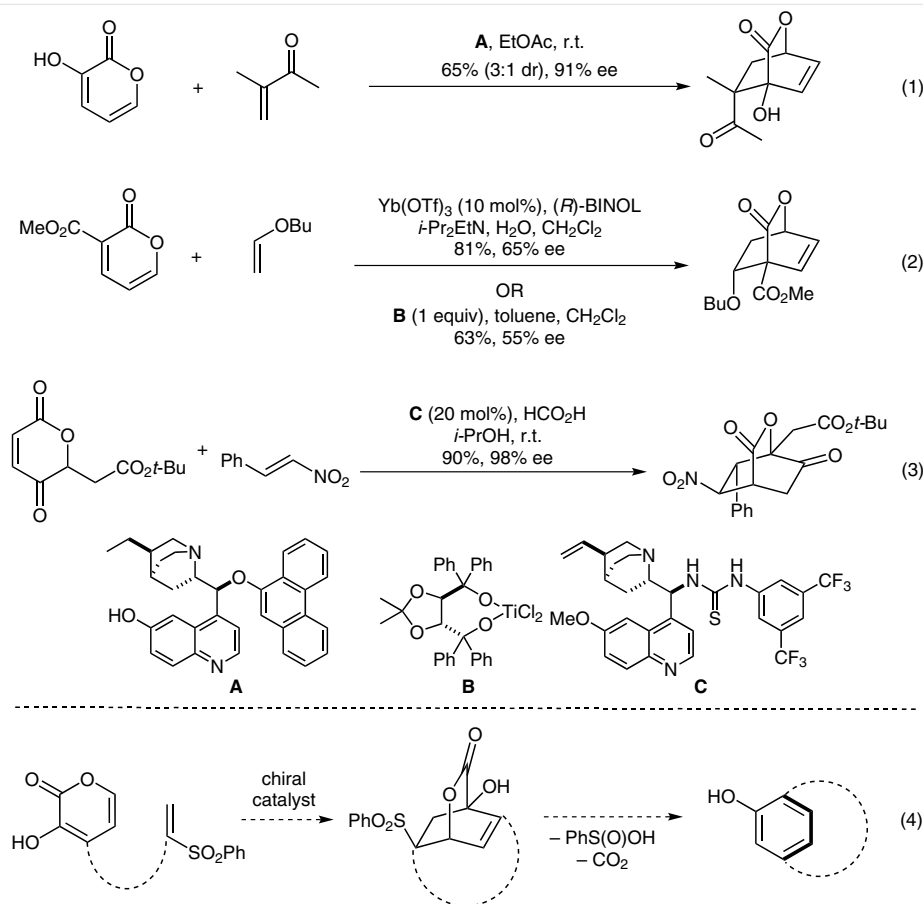
Scheme 4 Enantioselective pyrone Diels–Alder reactions
