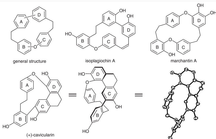
Figure 1 Selected macrocyclic bis(bibenzyl) natural products
