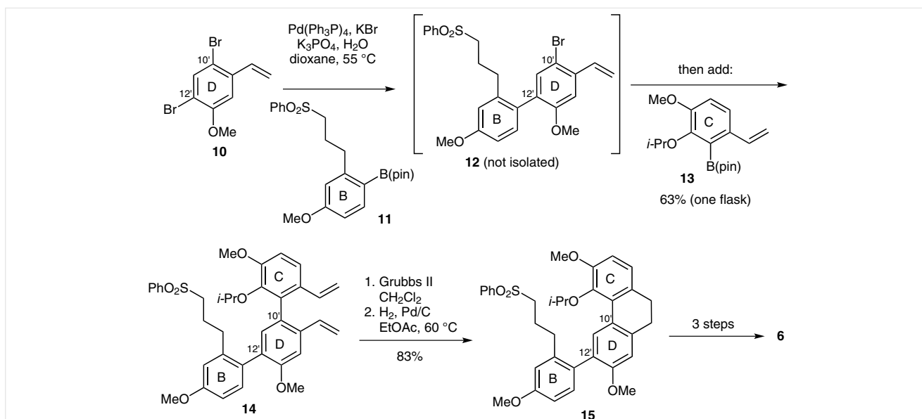
Scheme 5 Suzuki reactions for cavicularin
