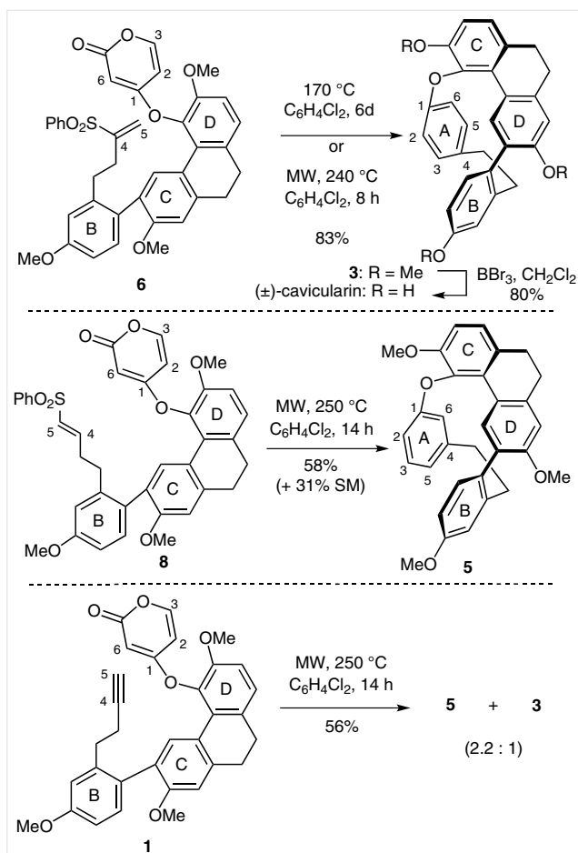
Scheme 6 Synthesis of (±)-cavicularin
