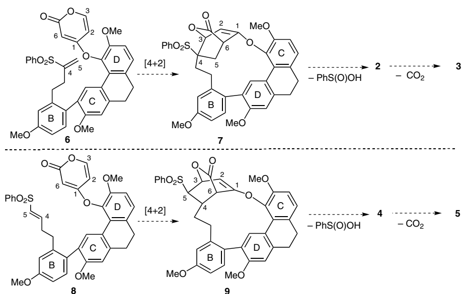
Scheme 3 Vinyl sulfones as alkyne equivalent dienophiles
