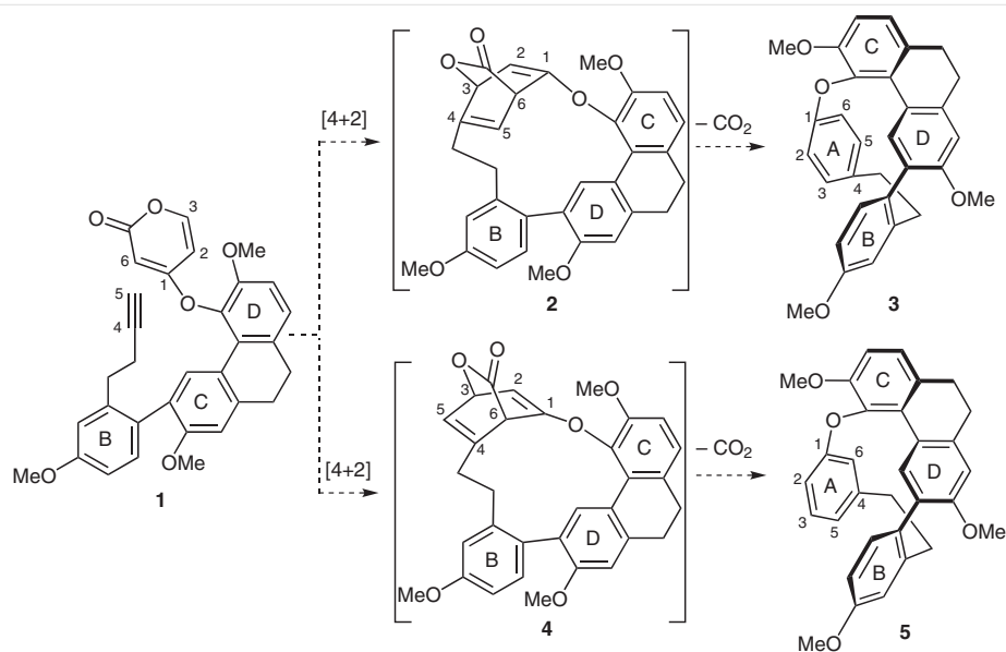
Scheme 2 Pyrone-alkyne Diels-Alder reaction for cavicularin
