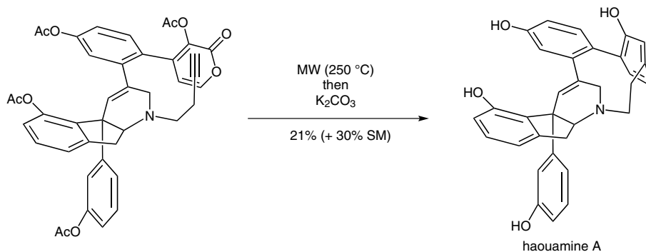
Scheme 1 Synthesis of hauuamine A developed by Baran and Burns
